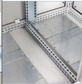
Interior partition profile
