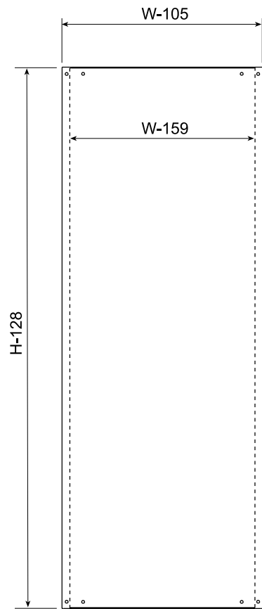
Mounting plate
