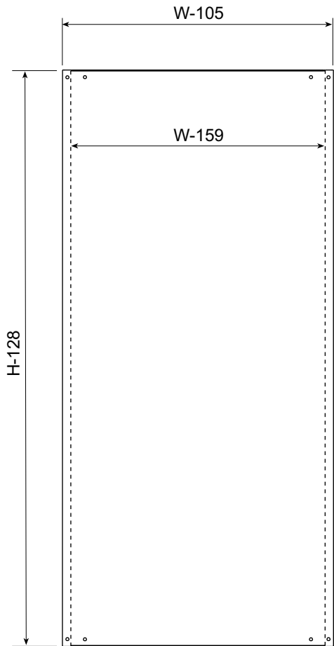
Mounting plate
