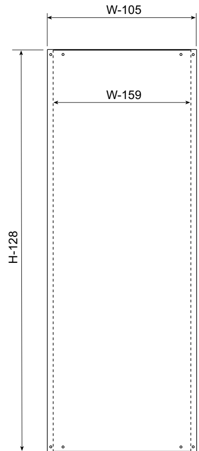
Mounting plate
