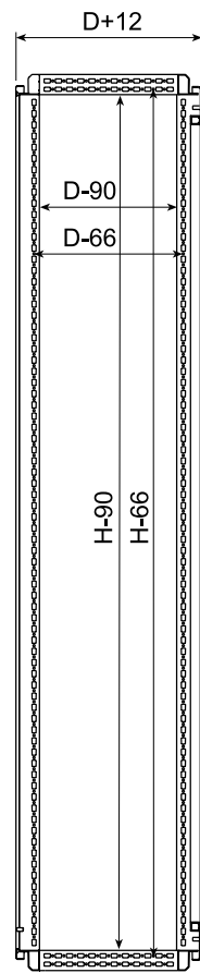
Ground plan section
