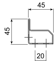
Profile
